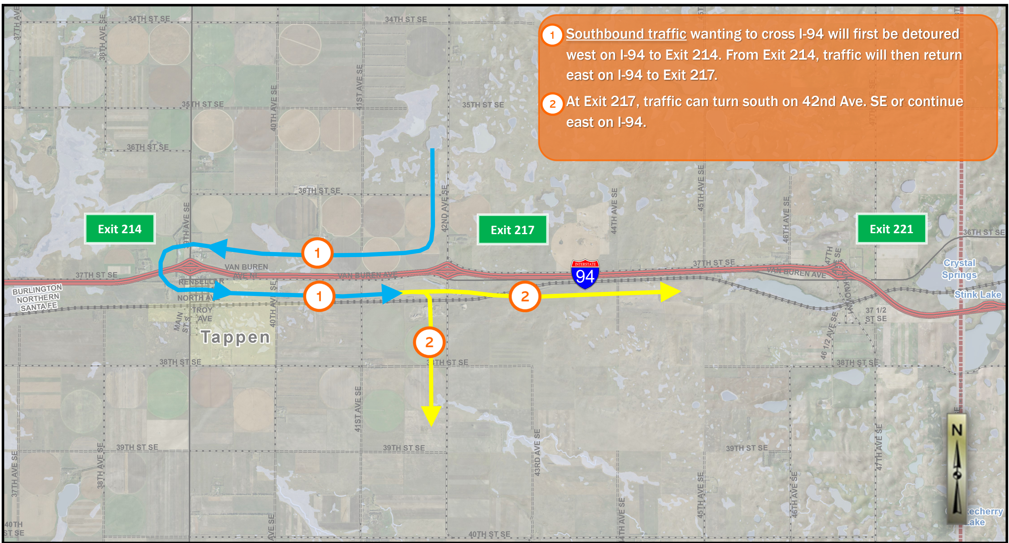
Detour plan for 42nd Ave. SE crossroad traffic (southbound)
