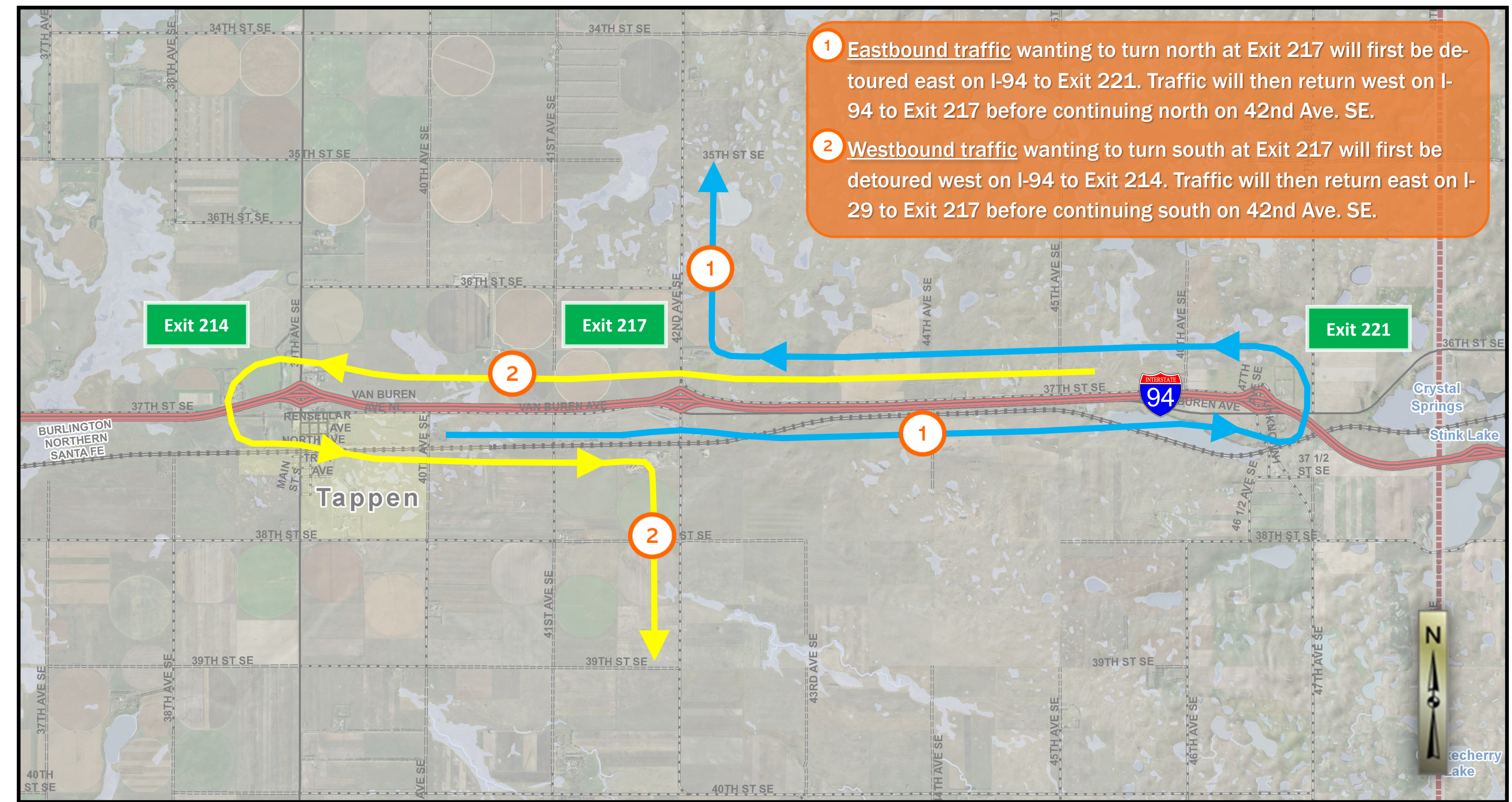
Detour plan for traffic exiting interstate at Exit 217
