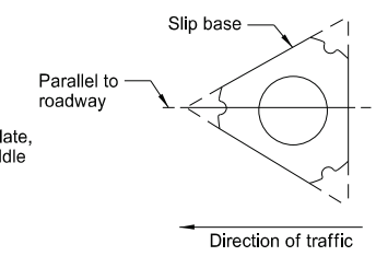
Slip Base Placement Detail
