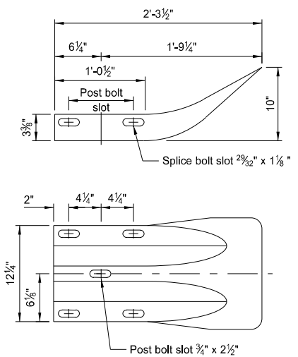
W BEAM END SECTION (FLARED)
