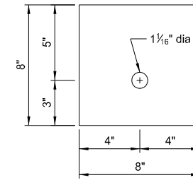
BEARING PLATE
