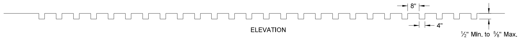
SAW SLOTTED RUMBLE STRIP DETAIL
