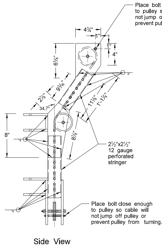
Detail B
