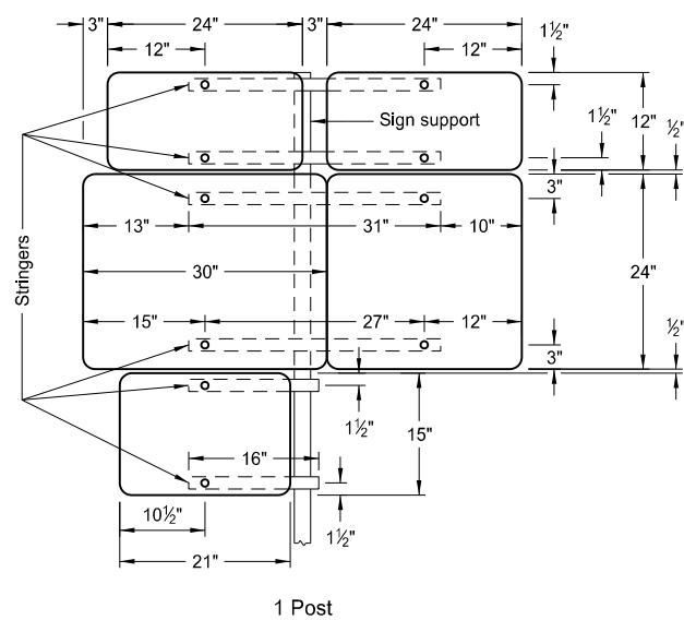
1 Post
