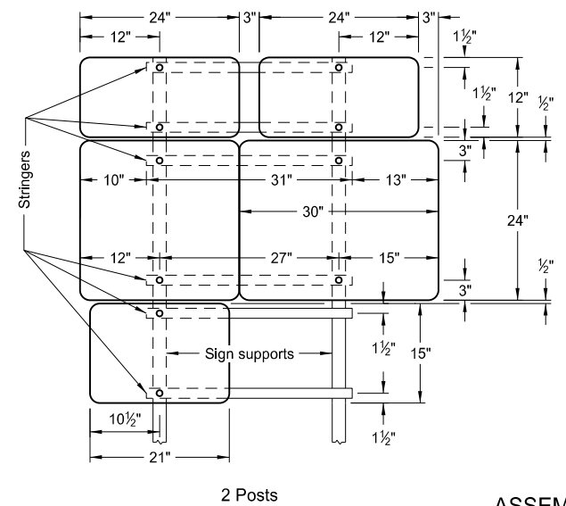
ASSEMBLY 384
