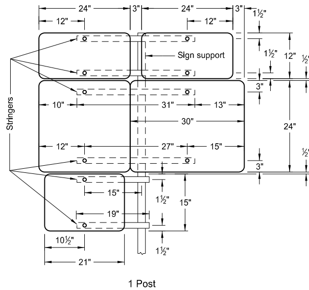
1 Post
