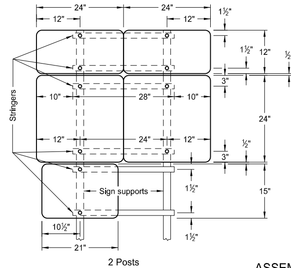
ASSEMBLY 383
