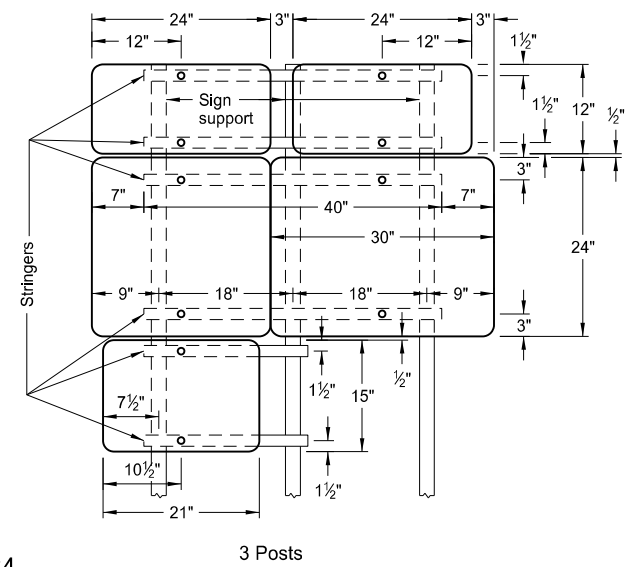
3 Posts
