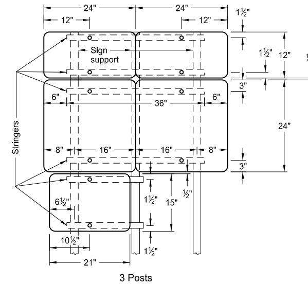
3 Posts
