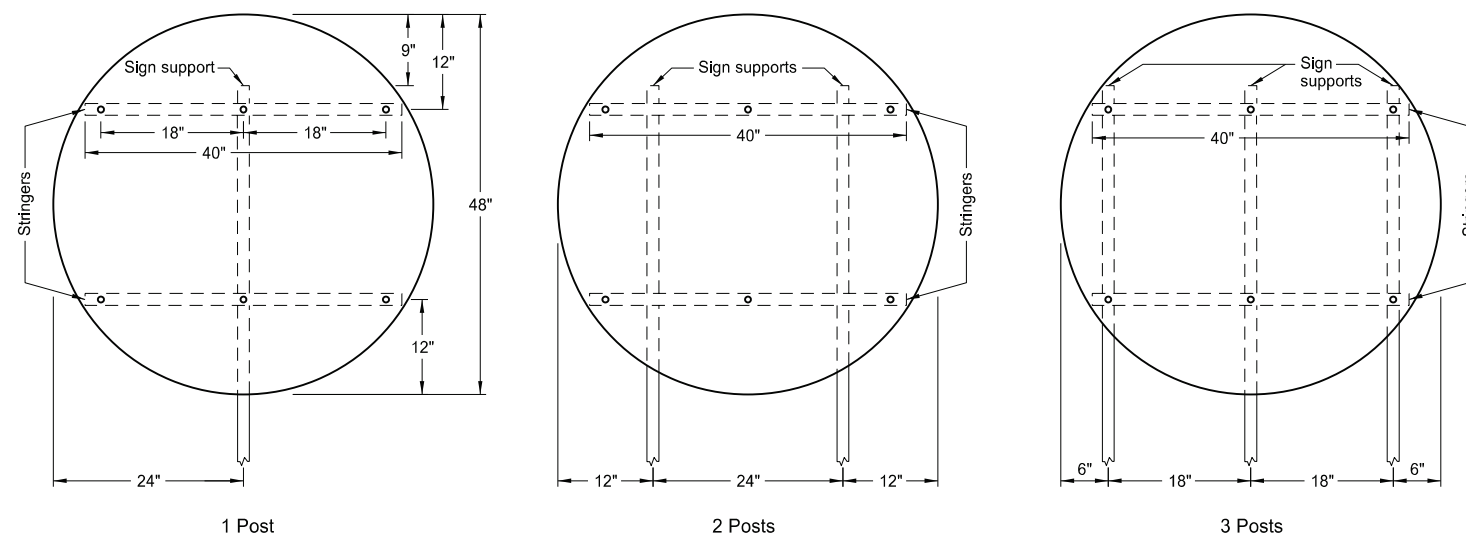
ASSEMBLY NO. 64
