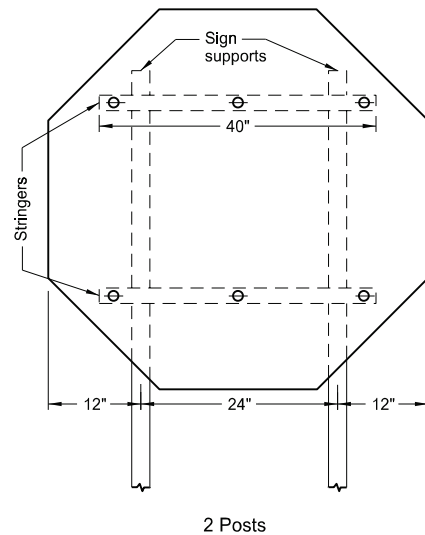
Assembly No. 3
