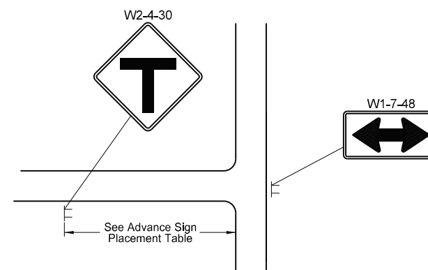
Roadway Termination with T-Intersection Type C
