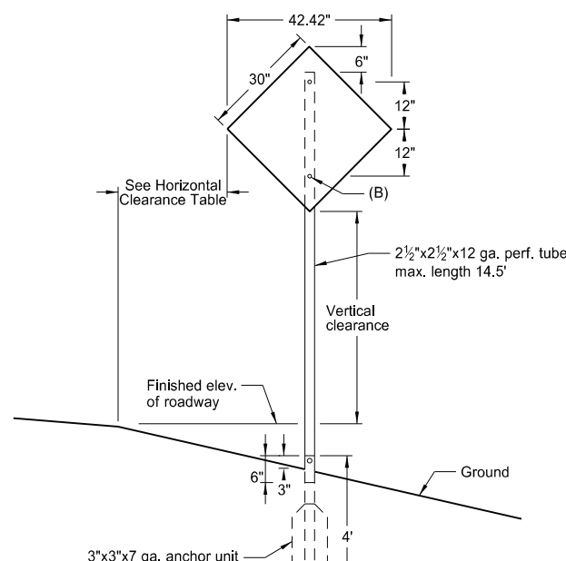
Assembly Detail for 30" Signs
