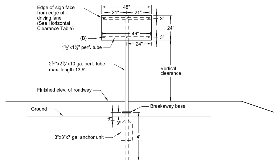
Assembly Detail for Directional Arrow Signs
