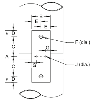
Perforated Fuse Plate
