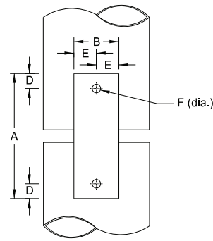
Hinge Plate
