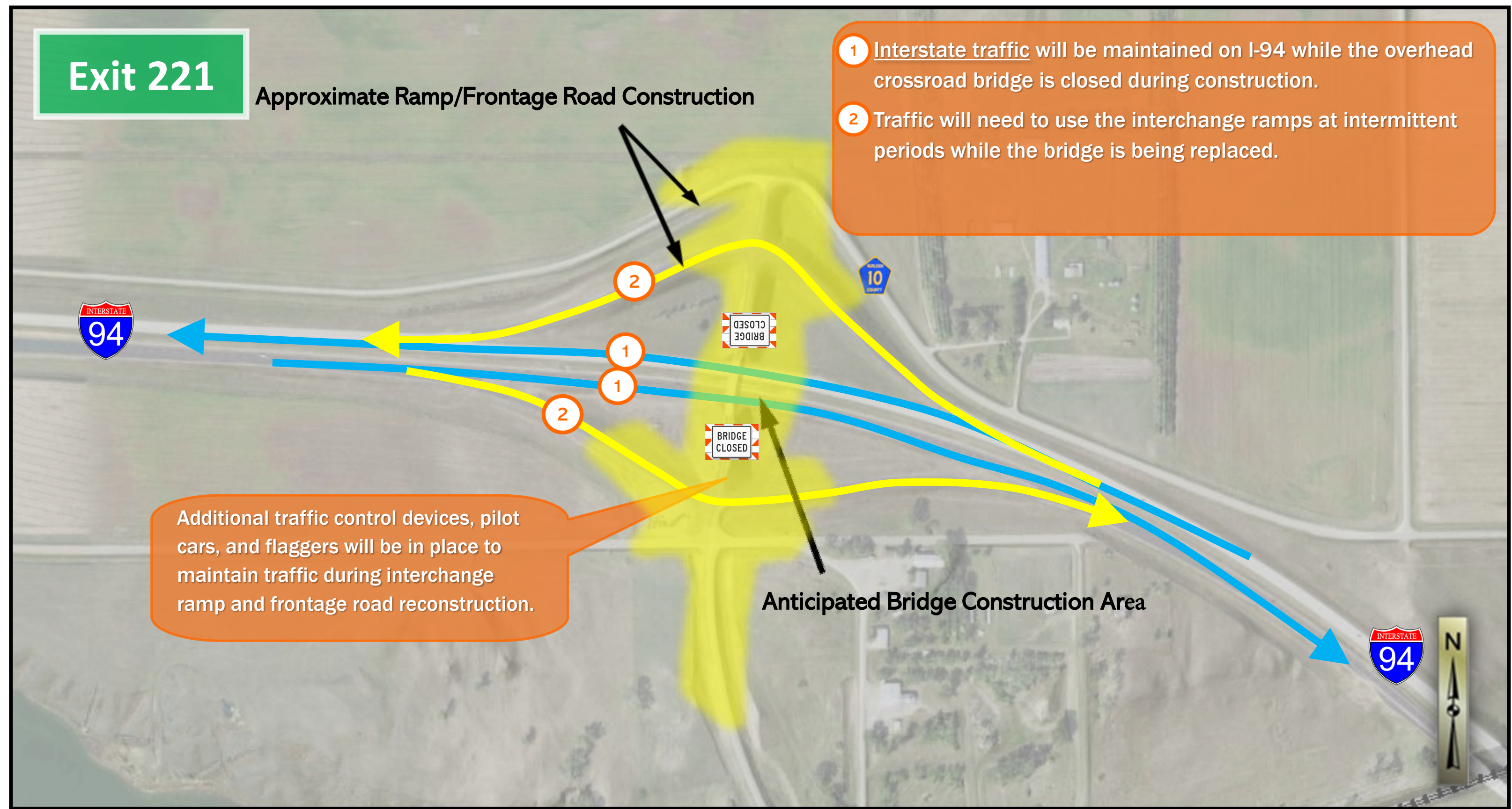
Detour plan for interstate thru-traffic
