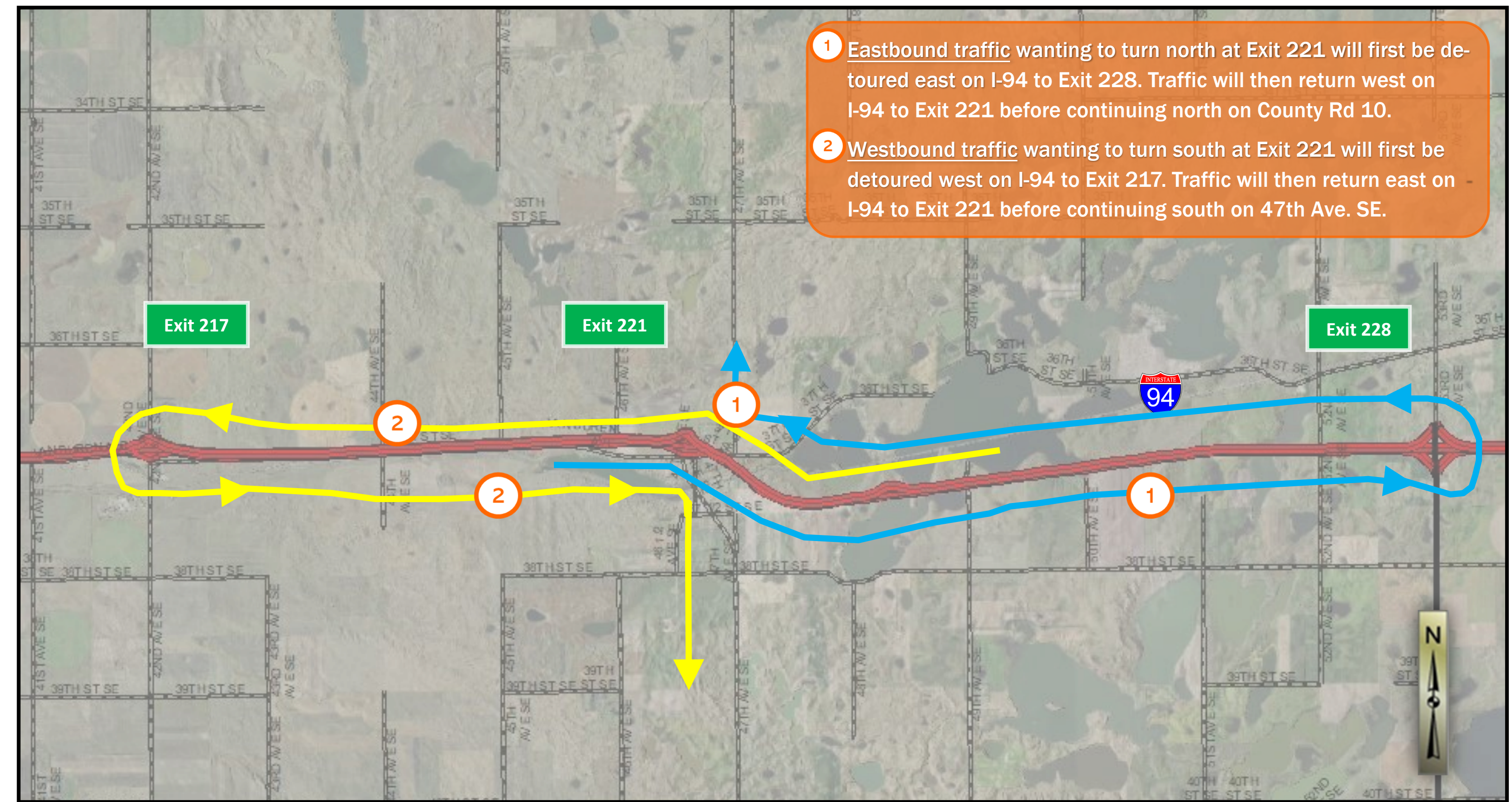
Detour plan for traffic exiting interstate at Exit 221
