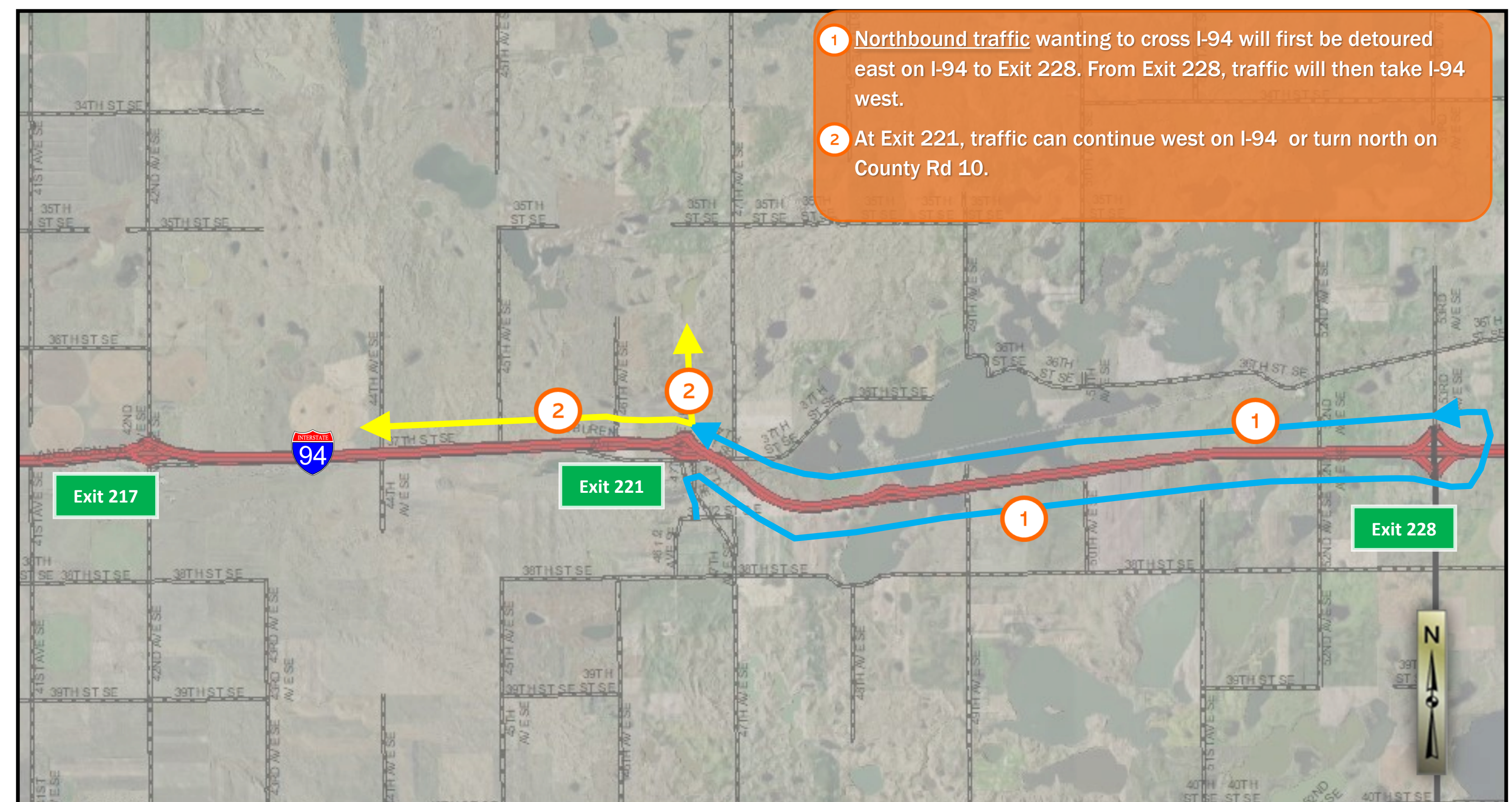
Detour plan for 47th Ave. SE crossroad traffic (northbound)
